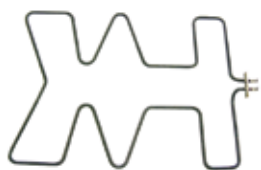
RESISTENCIA 3000W 400V HEATING ELEMENT 3000W/400V Cod. AMBACH: 5060825601 Cod. IBERITAL: 42430
